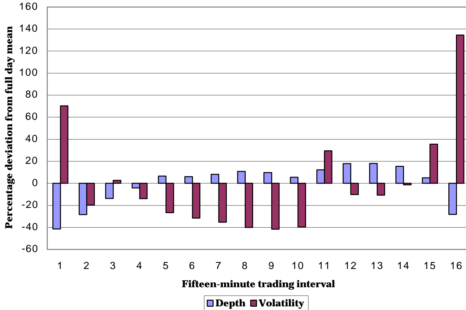
Figure 1.: Intraday Pattern in depth and volatility
